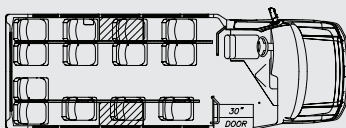
AeroLite 210 13 Passenger
